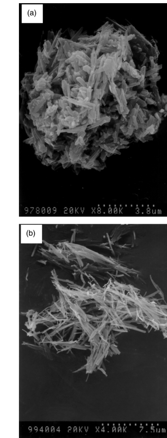
Fig. 1 SEM pictures of APDAP150 synthesized at 150 (a) and 120 °C (b).
