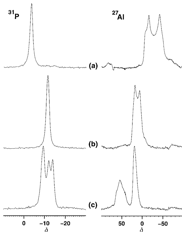
Fig. 5 ^{31}\text{P} and ^{27}\text{Al} MAS NMR spectra of APDAP150. As-synthesized (a), heated at 150 °C (b) and heated at 200 °C (c).
