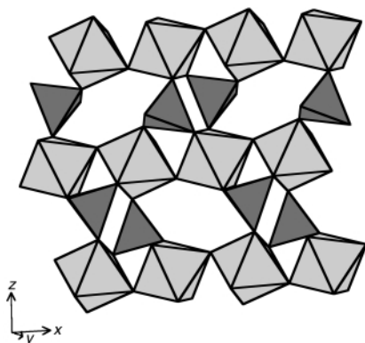
Fig. 4 Polyhedral drawing of the aluminophosphate layer of APDAP150 (dark gray, \text{PO}_4 tetrahedron; pale gray, \text{AlO}_6 octahedron).
